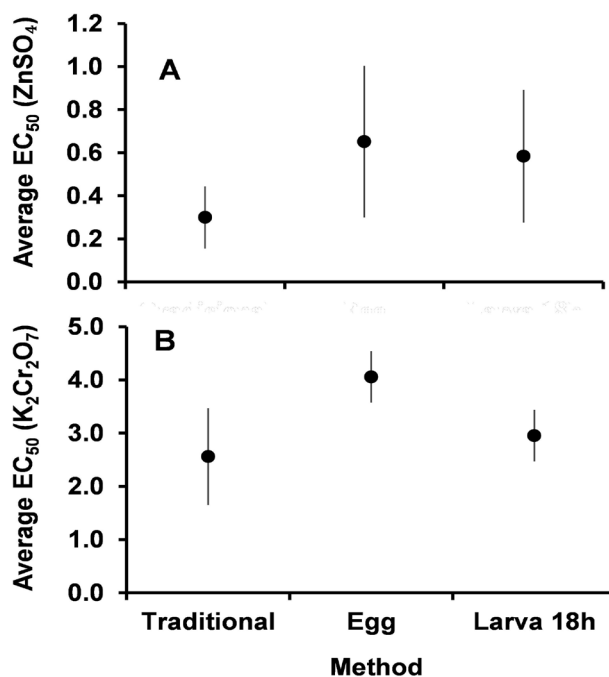
Figure 5. Mean values (point) and standard deviation (line) of EC 50 for ZnSO 4 ·7H 2 O (A) and K 2 Cr 2 O 7 (B) estimated in the traditional way (counting method) and by measuring the larvae using the effect percentages obtained in based on egg and larval size at 18h (positive controls). Based on 15 tests carried out between the years 2017 to 2019.
